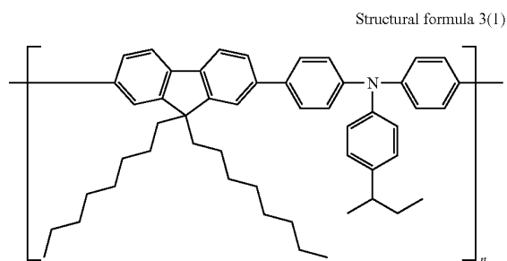
Chemical formula 10
