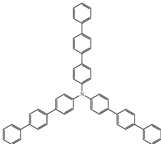
Compound 1 (23)
