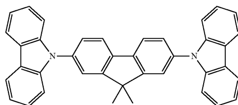
Compound 1(58)
