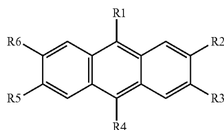
Chemical formula 6
