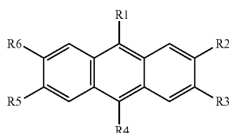
Chemical formula 2
