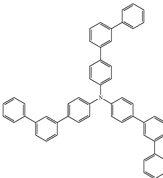
Compound 1(22)
