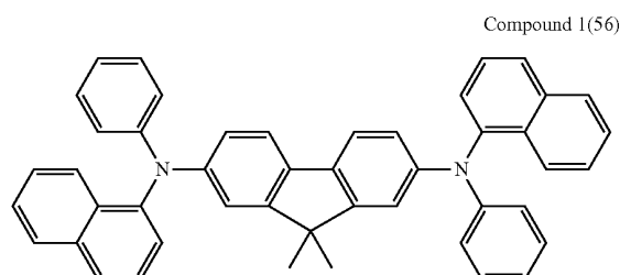
Chemical formula 11
