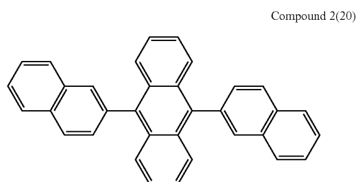
Chemical formula 13
